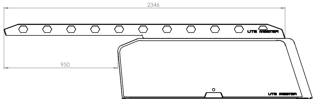
SIDE VIEW CANTILEVER ROOF RACK
