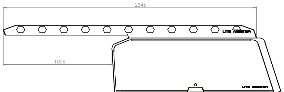
SIDE VIEW CANTILEVER ROOF RACK (X-Terrain)
