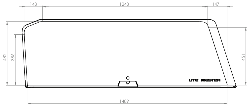
SIDE VIEW DOORS DOWN
