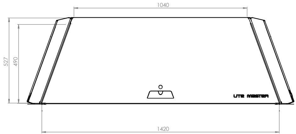
REAR VIEW DOORS DOWN
